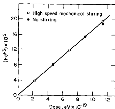
Fig. 1. Ferric ion production in the Fricke dosimeter as a function of dose for 102 MeV \text{C}^{+6} ions.
